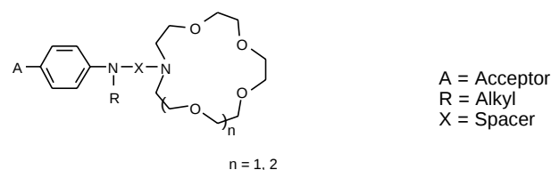
Scheme 1 Spacer-Chromionophores
